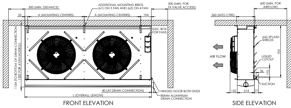
FRONT ELEVATION
