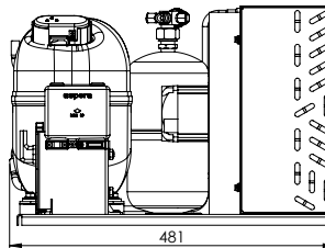
UNJ2192GK - UNJ2212GK
