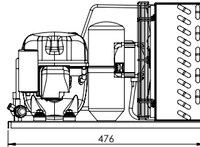
UNJ2192GK - UNJ2212GK
